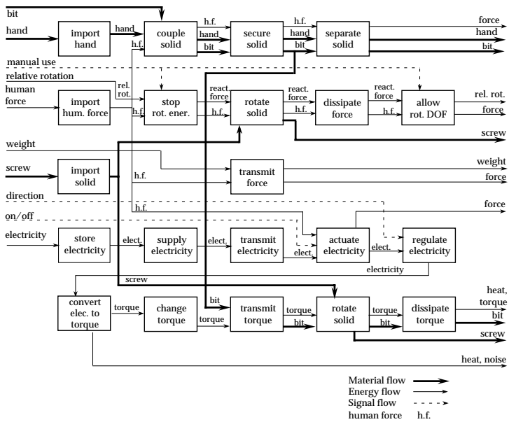
Figure 4 The functional model for a power screwdriver.
