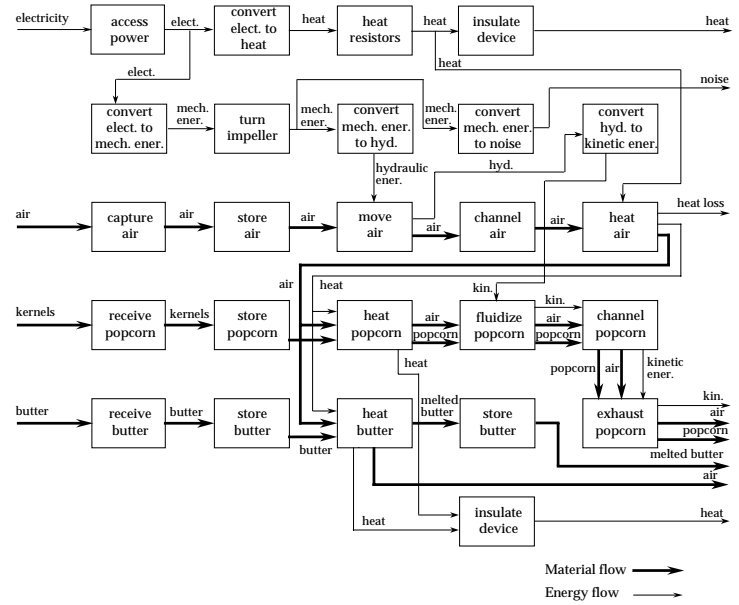
Figure 6 Functional model of the hot air popcorn popper generated without a structured vocabulary.
