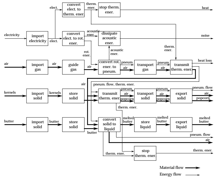
Figure 7 Functional model of the hot air popcorn popper generated using the functional basis.
