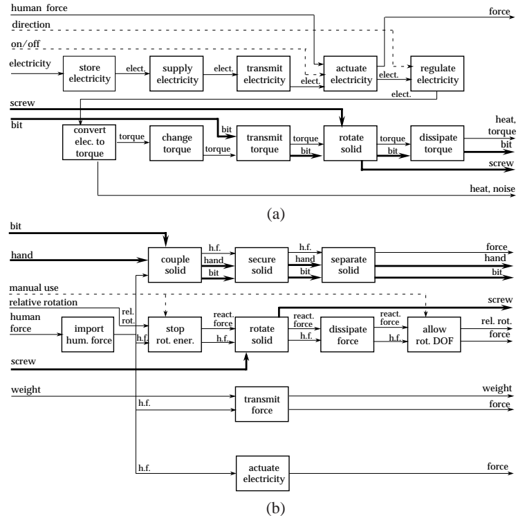
Figure 3 Examples of two function chains for a power screwdriver. (a) A sequential function chain for the flow of electricity and torque . (b) A parallel function chain for the flow of human force .
