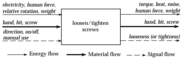
Figure 2 A Black Box model for a power screwdriver.
