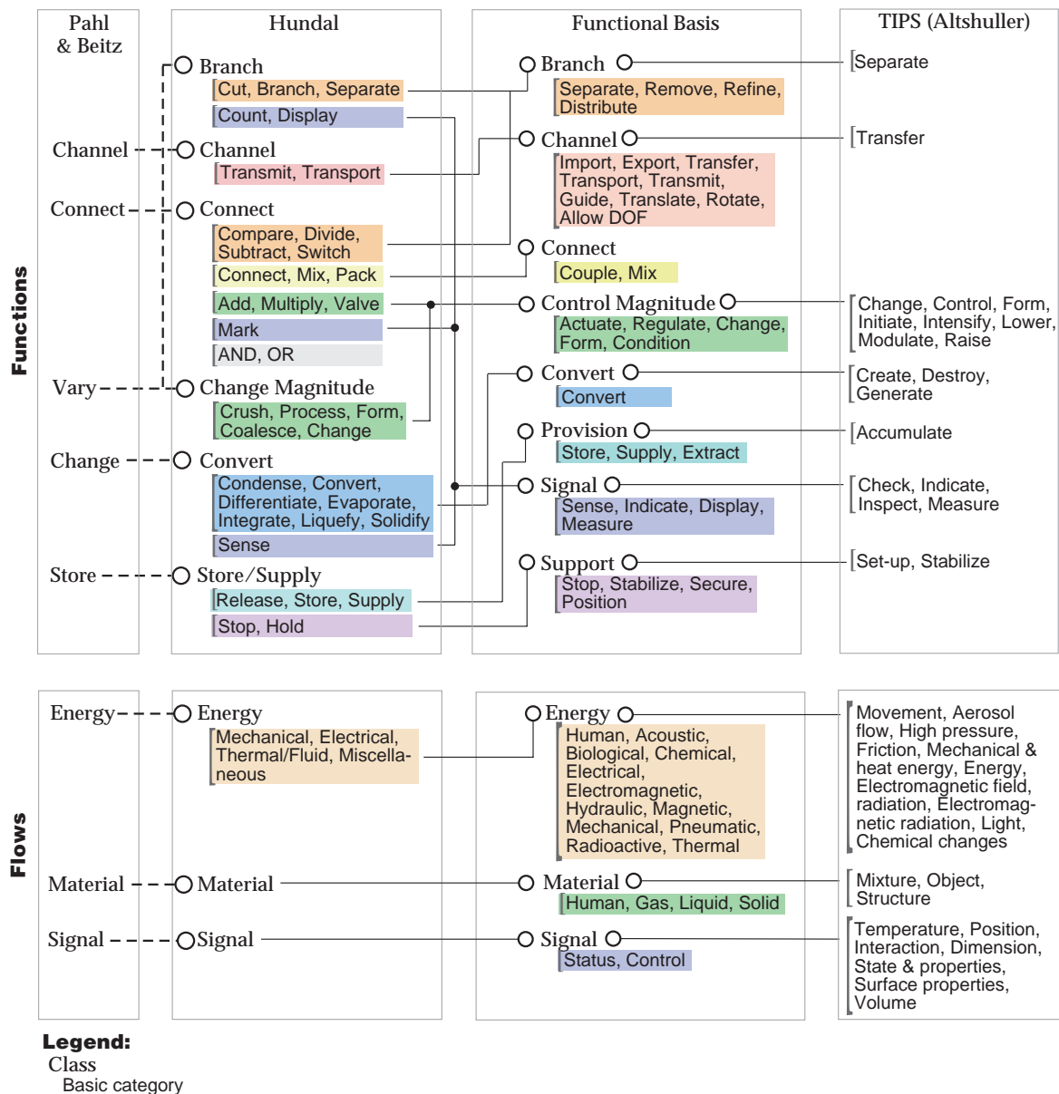
Figure 1 Comparison of earlier function taxonomies with the functional basis. TIPS 30 function descriptions are also represented as functions and flows and shown to be subsumed by the functional basis.
